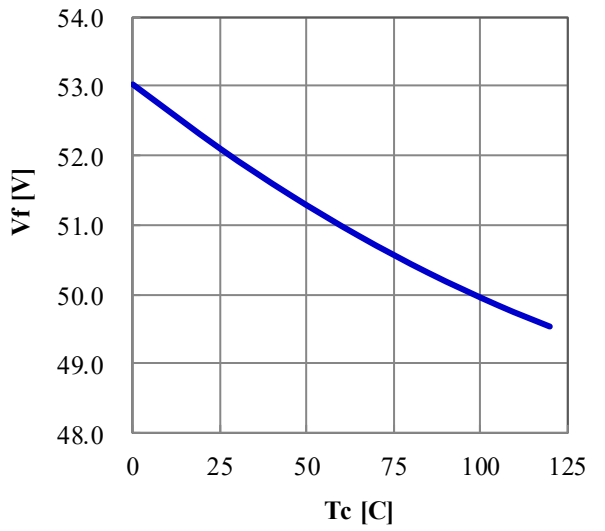
Case Temperature vs. Forward Voltage If=2250mA
