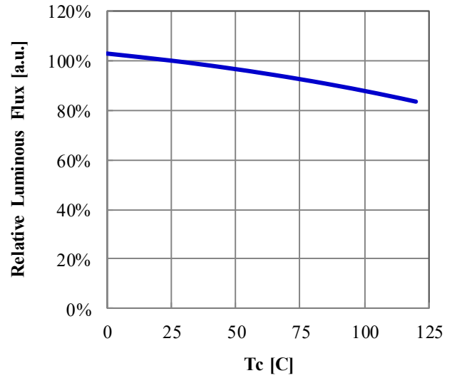
Case Temperature vs. Relative Luminous Flux If=2250mA
