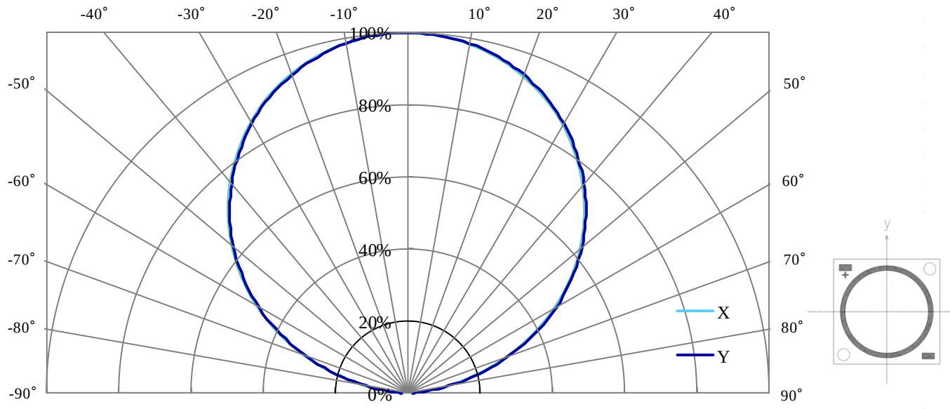
Radiation Characteristic
