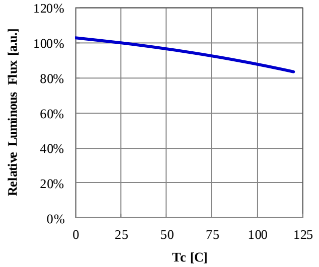
Case Temperature vs. Relative Luminous Flux If=1620mA
