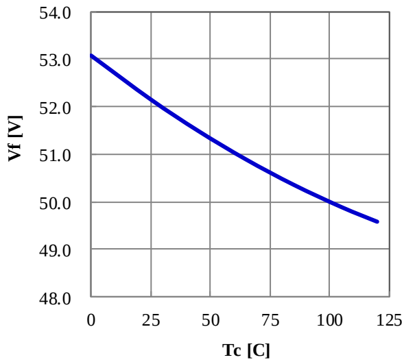
Case Temperature vs. Forward Voltage If=1620mA
