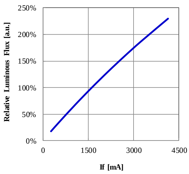
Forward Current vs. Relative Luminous Flux Tc=25C
