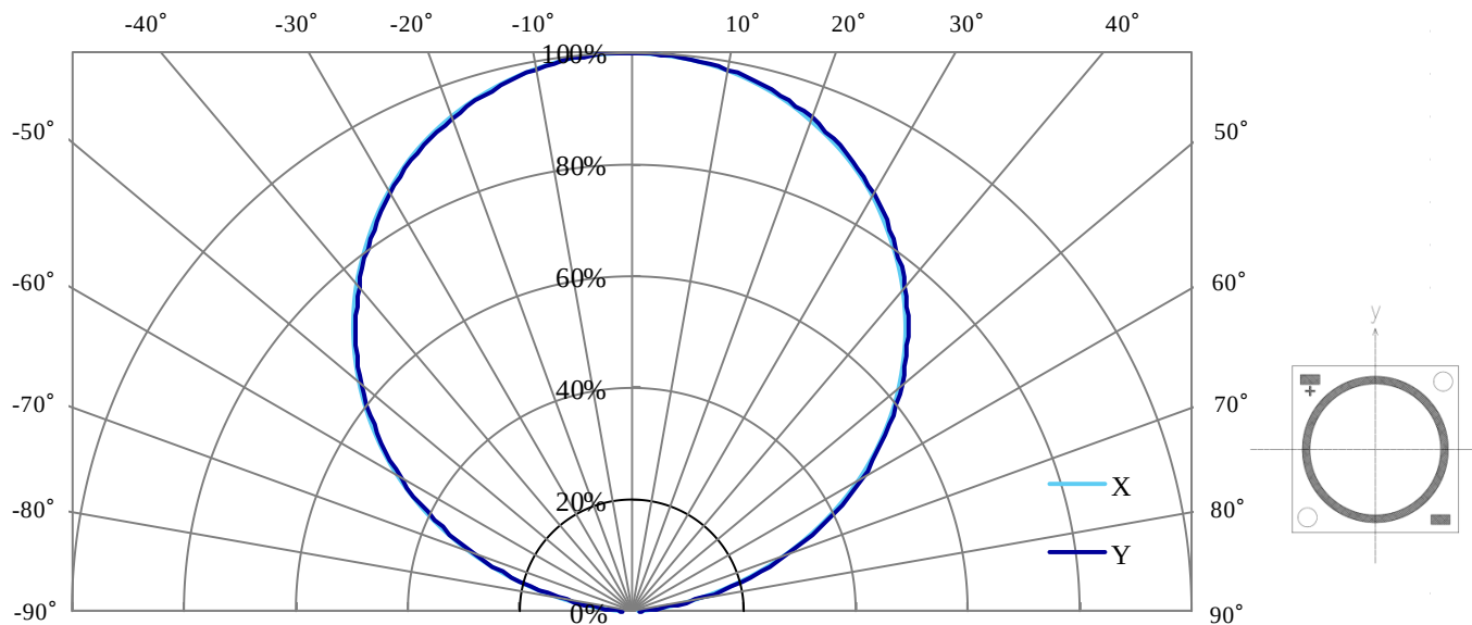
Radiation Characteristic
