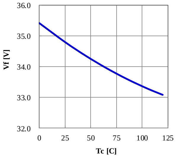
Case Temperature vs. Forward Voltage If=1080mA
