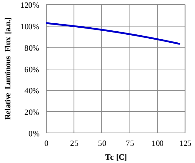
Case Temperature vs. Relative Luminous Flux If=1080mA
