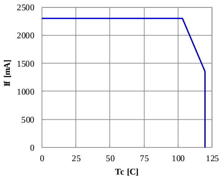
Case Temperature vs. Allowable Forward Current
