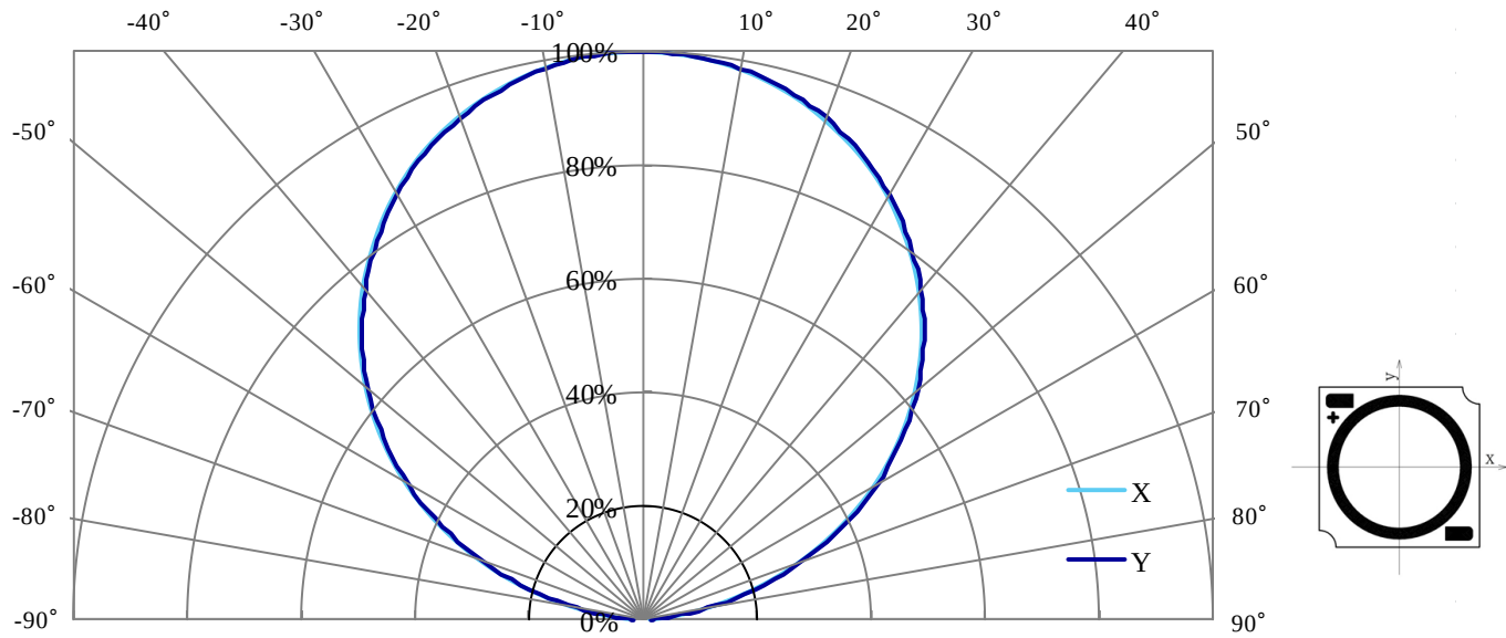
Radiation Characteristic
