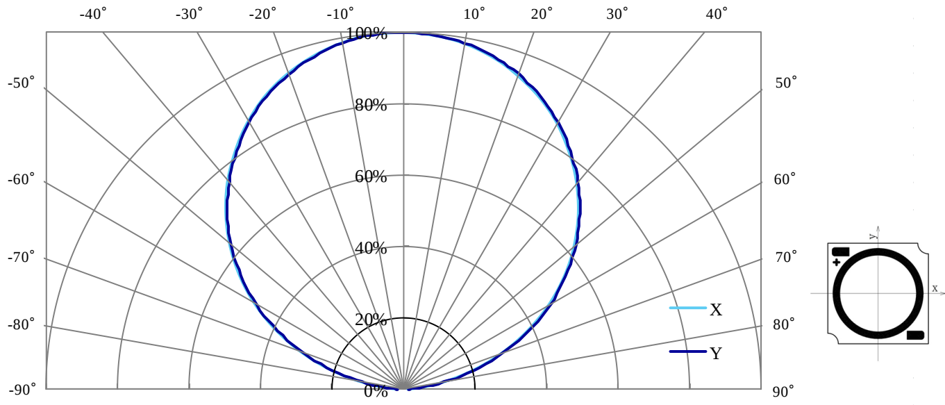
Radiation Characteristic
